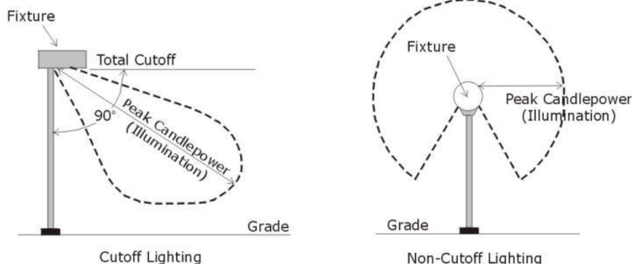
Figure 8-A: Illustration of cutoff lighting versus non-cutoff lighting
