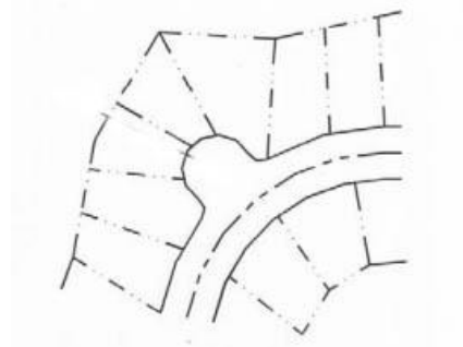
Figure 16-G: Illustration of a knuckle street configuration
